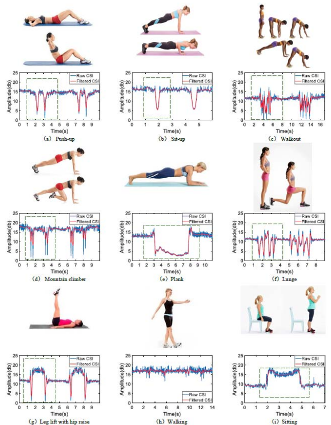
Signal amplitude patterns for 9 activities
